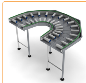
Virage 180° 1650x1075x870
